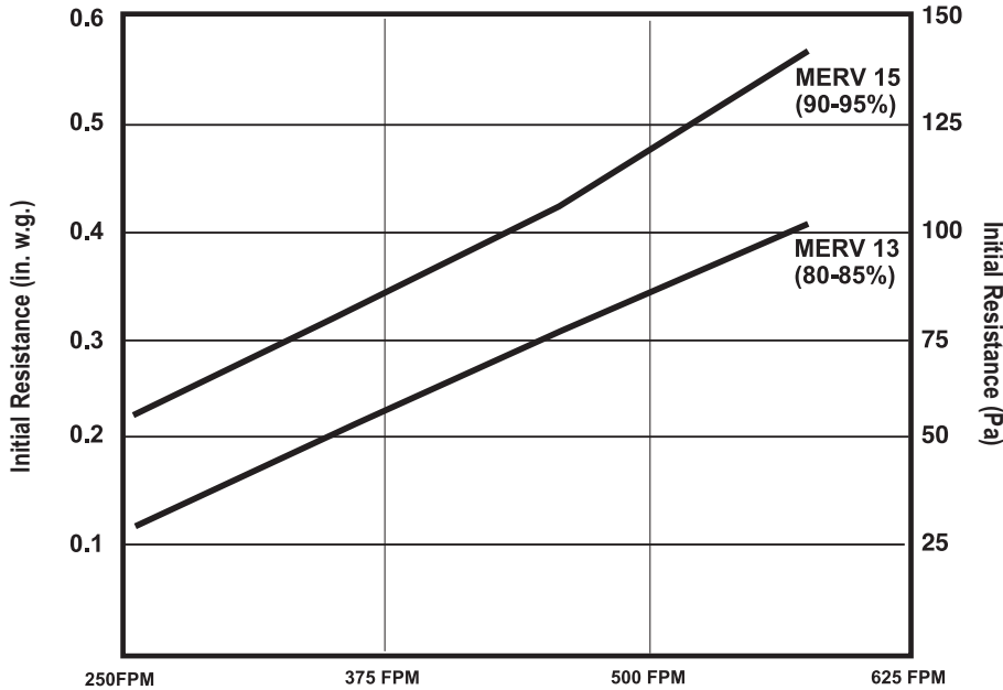
Initial Resistance vs. Airflow
