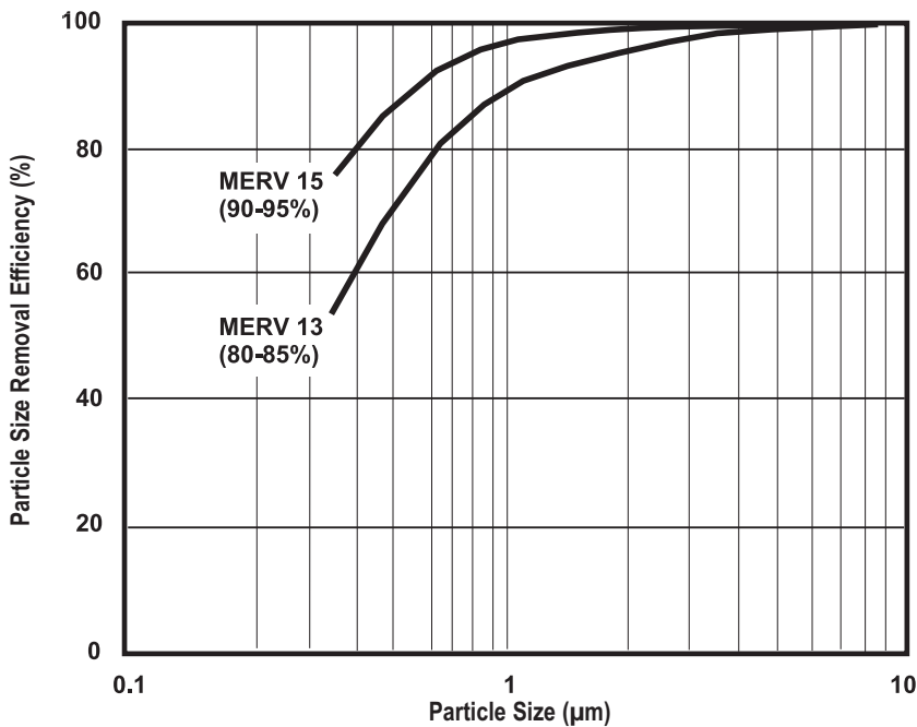
Composite Minimum Efficiency Curve
