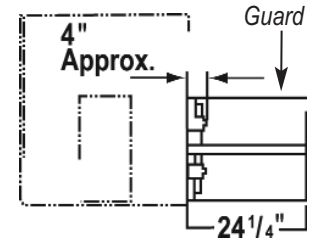
Figure 7. Explosion Vent Guard
