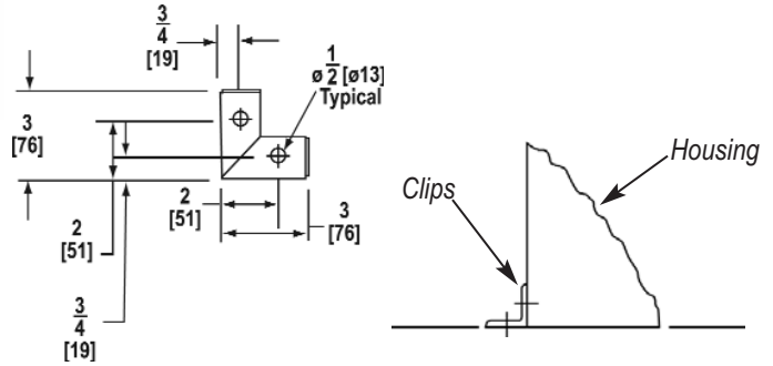
Figure 2. Anchoring—Funnel Bottom
