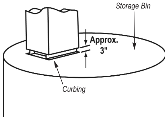
Figure 5. Bin Vent
