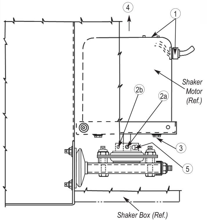
Figure 8. Shaker Motor Replacement
