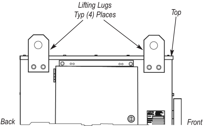
Figure 1. Lifting Lugs
