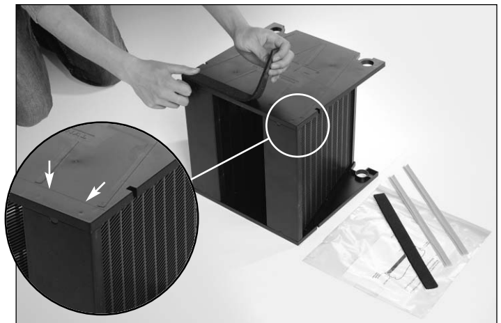
Step 2: Locate the gasket on the leaving air side of the half-cassette along the edge of the cassette side plate. A gasket location guide has been formed into the side plate. The gasket should be located to the outside of this line.
