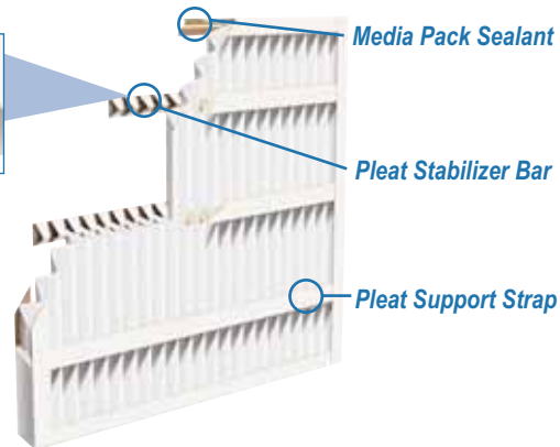
PerfectPleat® ULTRA 2" Construction
